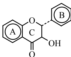
(10) Dihydroflavonol
