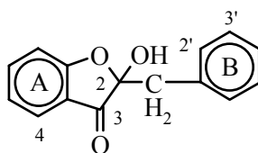
(6) Aurone hydrate or 2-Hydroxy-2-benzyl-3- coumaranone
