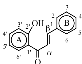
(1) 2'-Hydroxychalcone
