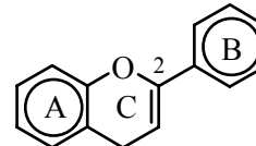
(14) 2-Flavene
