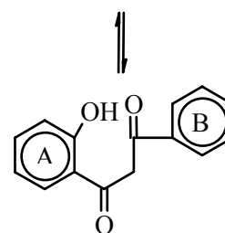
o -Hydroxy 1, 3-Dibenzoylmethane
