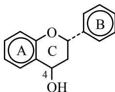
(13) 4-Hydroxyflavan
