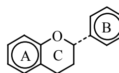
(11) Flavan
