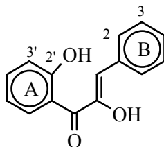
(2) a, 2'-Dihydroxychalcone
