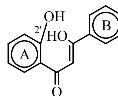
(2) , 2'-Dihydroxychalcone
