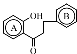
(4) 2'-Hydroxydihydrochalcone
