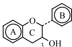
(12) 3-Hydroxyflavan
